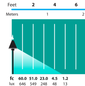
AL-18-SM Half Spread Photometrics 12ft (3.7m) diameter
