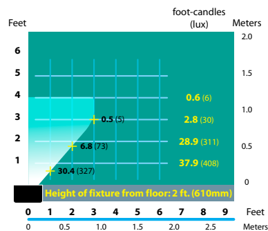
SL-18 Half Spread Photometrics
