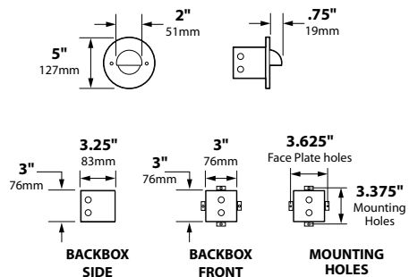
SL-24: Mounting Holes on all models 3.375" on center
