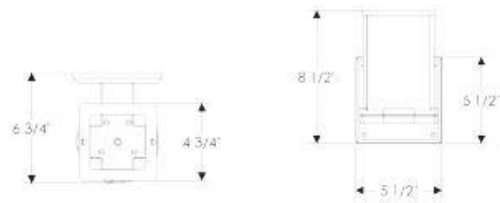
WS418 with E403 Square Escutcheon
