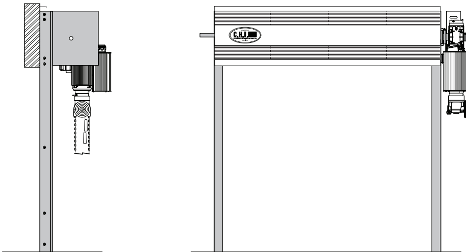
"Z" Guide: Steel or Masonry
