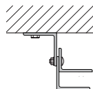
"Z" Guide: Steel or Masonry
