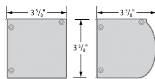
Non-ZIP 92 Motorized or Manual Operation square headbox (side view)
