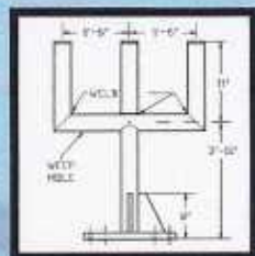
Instrument Stands
