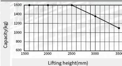
CAPACITY CHART
