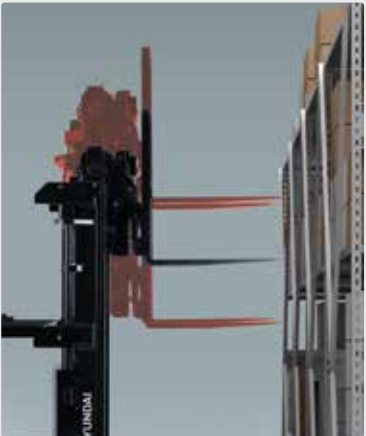
Beam Height Select There are 20 programmable presets with 10 load beam levels so operators can preselect the putaway and letdown fork positions. This standard feature works through the control handle not the dash.
