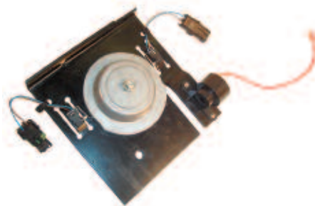
Fwd/Rvw Switch (No Handle) E-Z-Go PDS Electric 00+ OE OEM: 73180G03. FR-012
