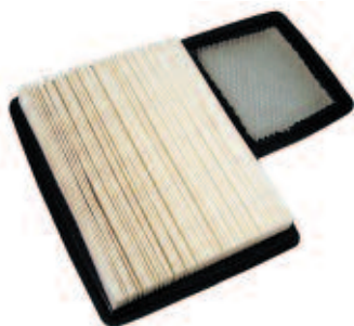
Air Filter, Yamaha G16-G22 4 Cycle Gas 96+ Paper element with expanded side screen. OEM: JN6-E4450-00; JN6-E4450-01. FIL-0001
