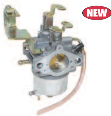
Carburetor, Yamaha 4 Cycle G16 OEM: JN6-14101-00. CARB-012A
