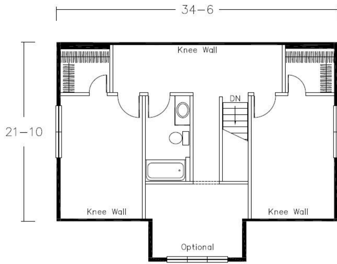
Craftsman Cottage Proposed Upper Level
