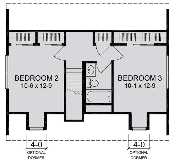
SUGGESTED SECOND FLOOR UNFINISHED (518 sq ft)
