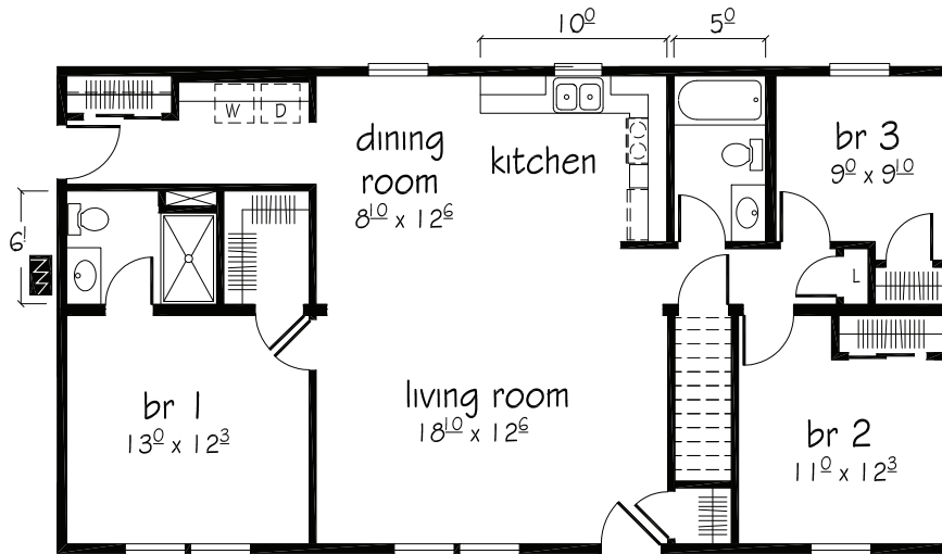
Logan I floor plan
