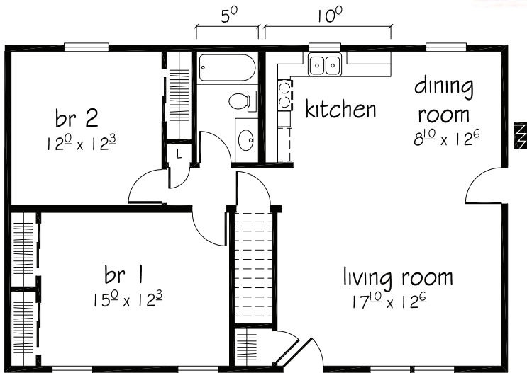
Mesa I floor plan 26'0" x 40'0" 1040 sq. ft.
