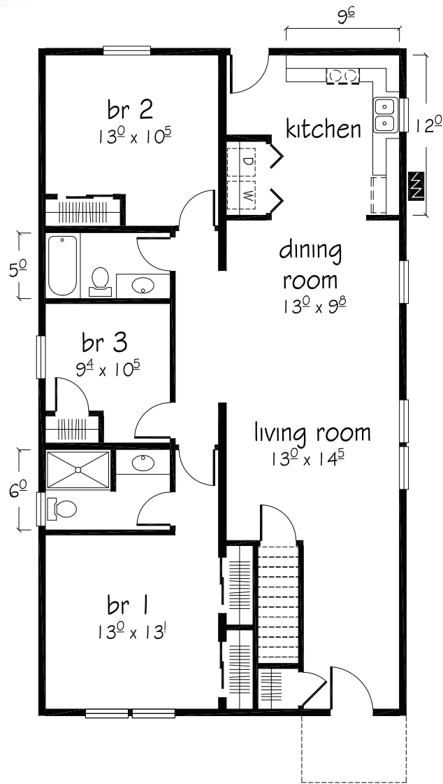
Willow I floor plan 27 6 x 50 0 1375 sq. ft.
