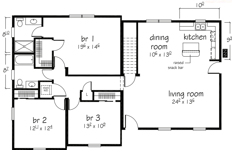
Crawford I floor plan 27 6 x 25 0 27 6 x 34/33 1622 sq. ft.
