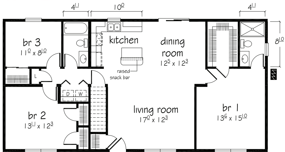
Lehigh I floor plan 26 0 x 52 0 1356 sq. ft.
