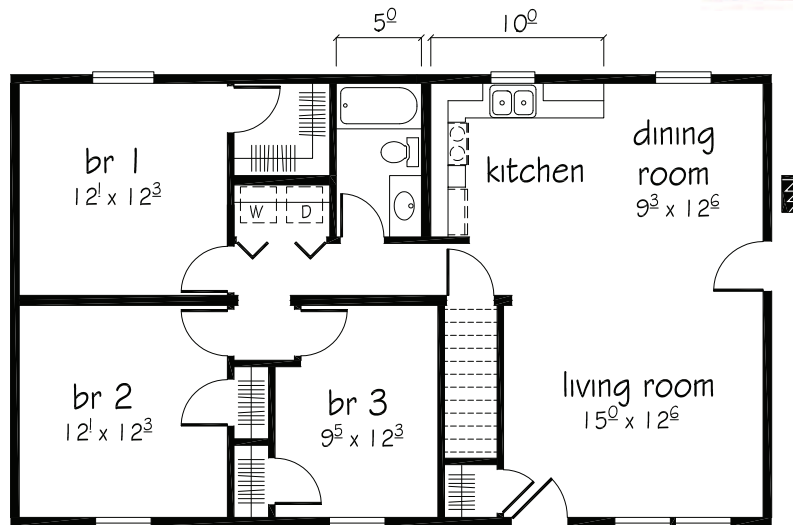
Fulton I floor plan
