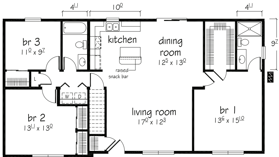
Lehigh II floor plan 26 9 / 27 6 x 52 0 1408 sq. ft.
