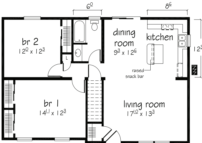
Mesa II floor plan 26'0" / 26'9" x 40'0" 1057 sq. ft.
