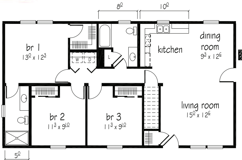
Essex I floor plan 26'0" x 48'0" 1248 sq. ft.
