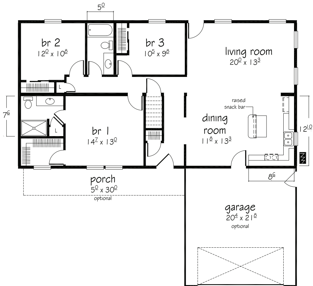
Freeport I floor plan 27 6 x 52 0 1417 sq. ft.
