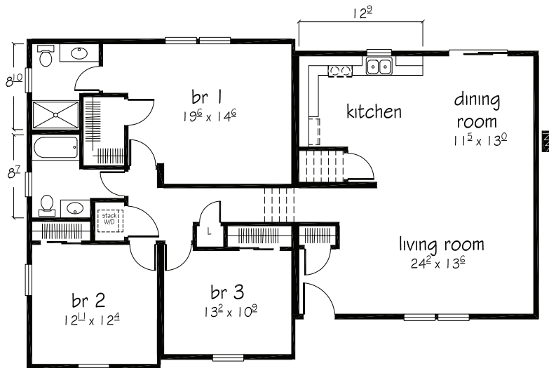
Crawford II floor plan 27 6 x 25 0 27 6 x 34/33 1622 sq. ft.
