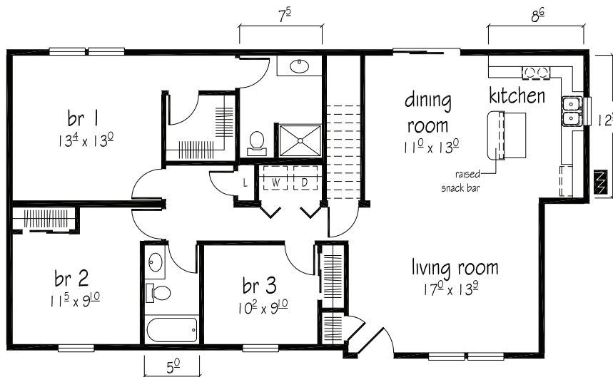
Essex II floor plan 27'6" / 26'9" x 52'48" 1352 sq. ft.
