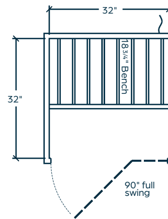
TOP DOWN VIEW
