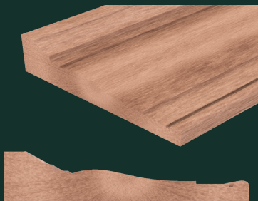
334 Interior Casing 1" x 3-3/4"
