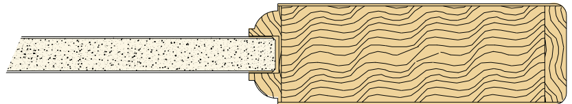
Flat Panel with Ovolo Sticking
