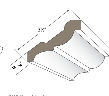
3 1/2" Bed Moulding AZM-28 Length: 16'
