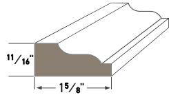
Shingle Moulding AZM-210 Length: 16'
