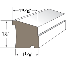
Sub Sill Nose AZM-6933 Length: 16'
