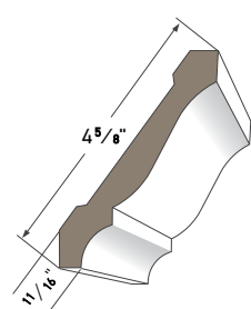
5" Crown AZM-47 Length: 16'
