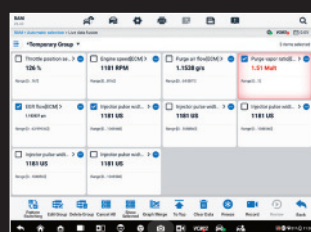
DATA-DRIVEN DIAGNOSTICS WITH ENHANCED PID ANALYSIS
