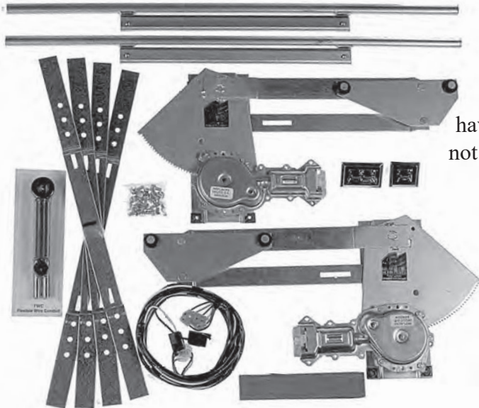
2416U-2C chrome switches shown
