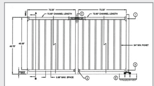
Guardrail Details
