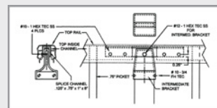
Intermediate Bracket
