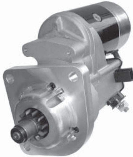
IMI - 25102-1140 12V CW 11 tooth
