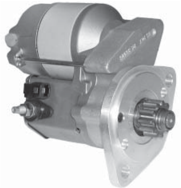
IMI - 215 12V CW 11tooth
