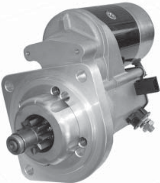
IMI - 25103-935 12V CW 9 tooth
