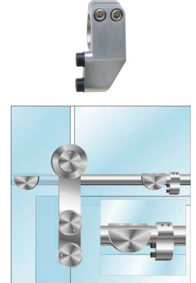
ESA-5R Right Door Stopper
