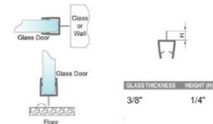
SGS One-Piece Bottom Rail With Clear Wipe for 3/8" Glass
