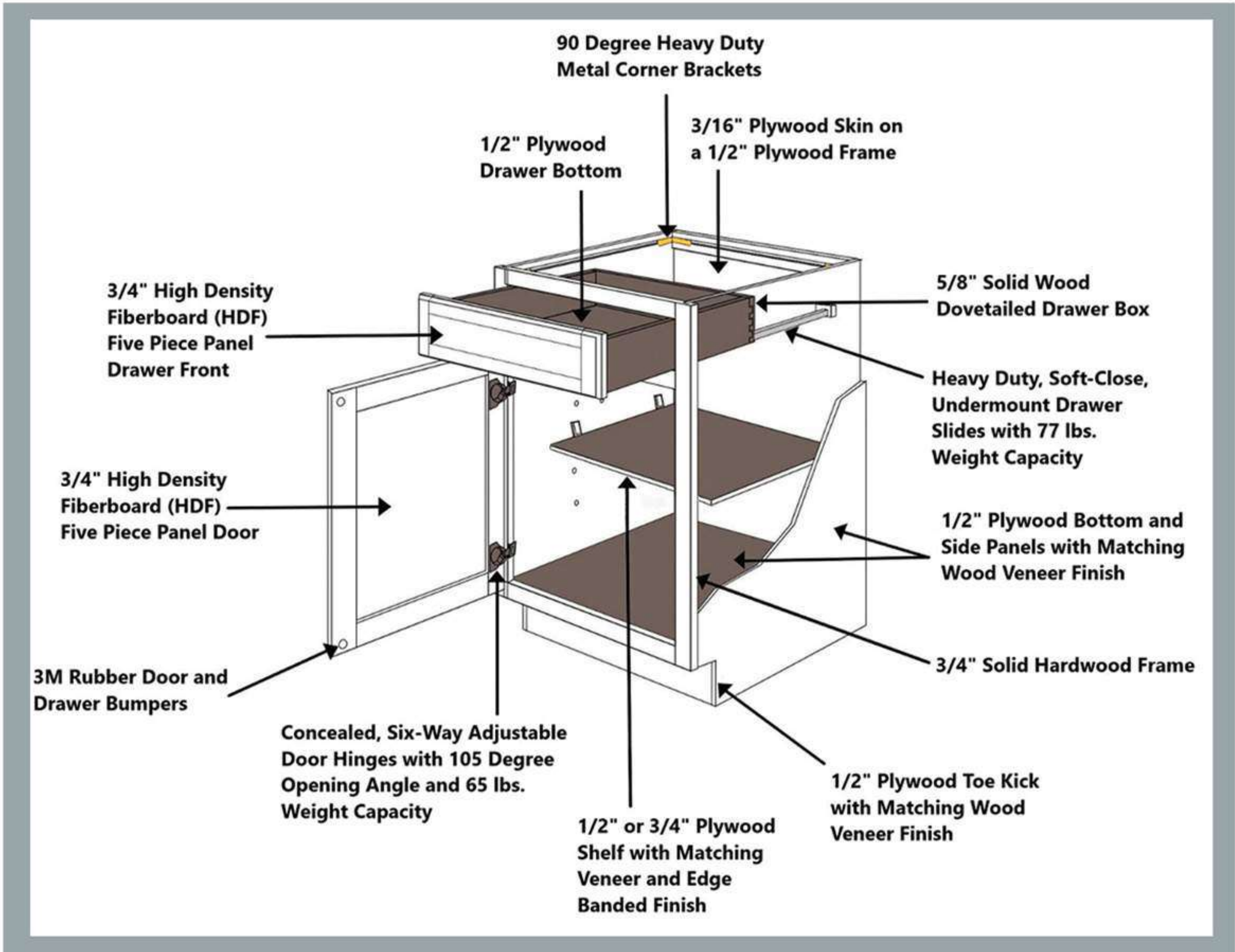
Base Cabinet Construction (HDF Door)
