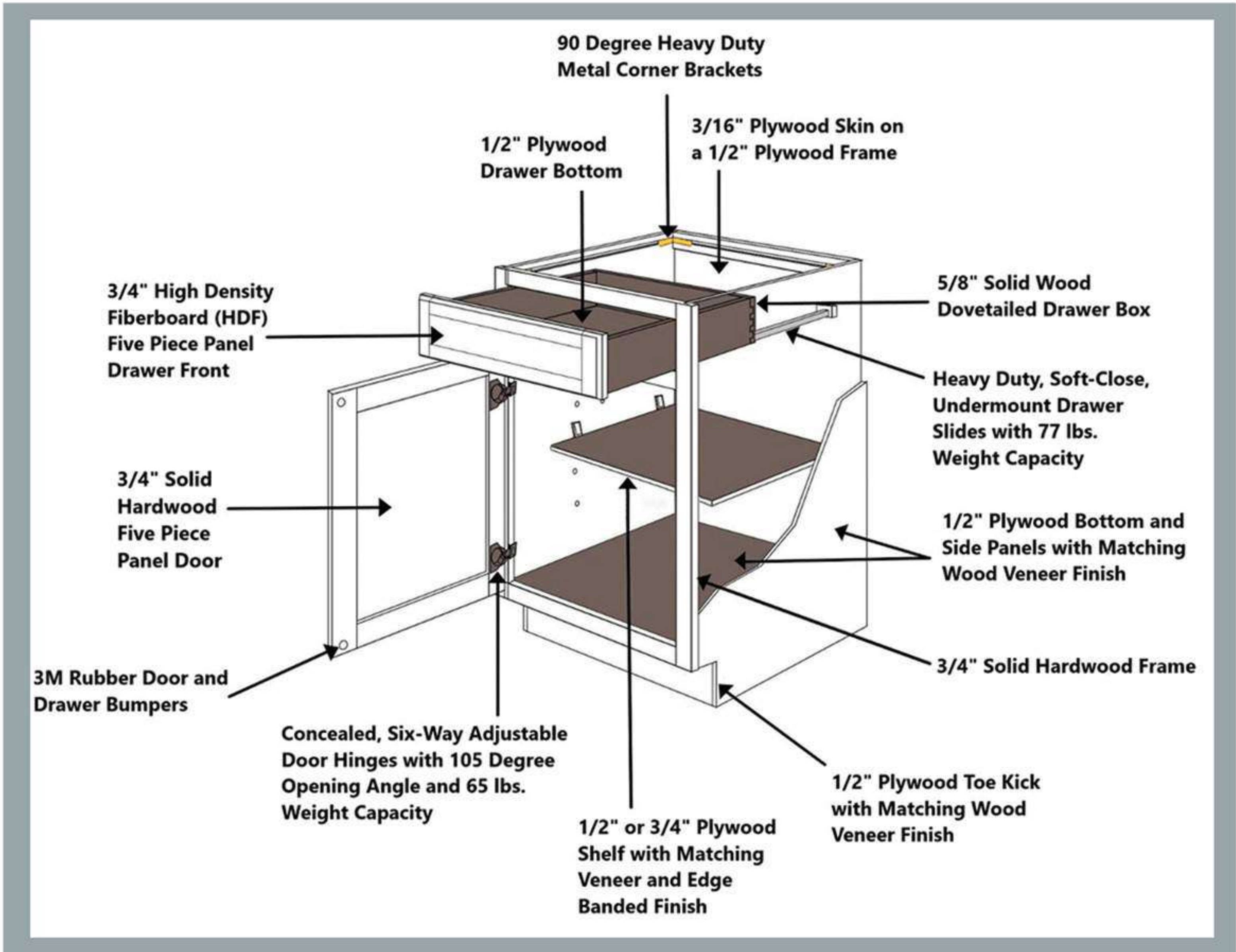
Base Cabinet Construction (Wood Door)
