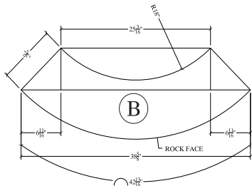
Fire Kit Cap Dimensions
