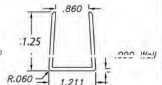
FW39108 Trim Channel
