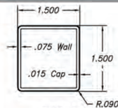
RW1140 1-1/2 x 1-1/2 Picket .075" Wall
