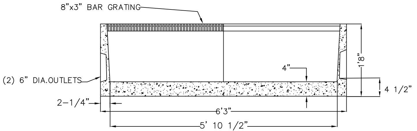
SIDE SECTION VIEW
