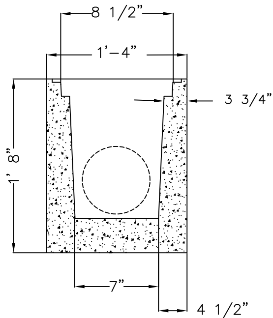
END SECTION VIEW
